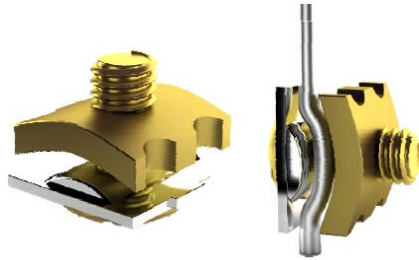
Furutech Patent Pending Clamp Contact Area Calculated Increase: 17.142%
