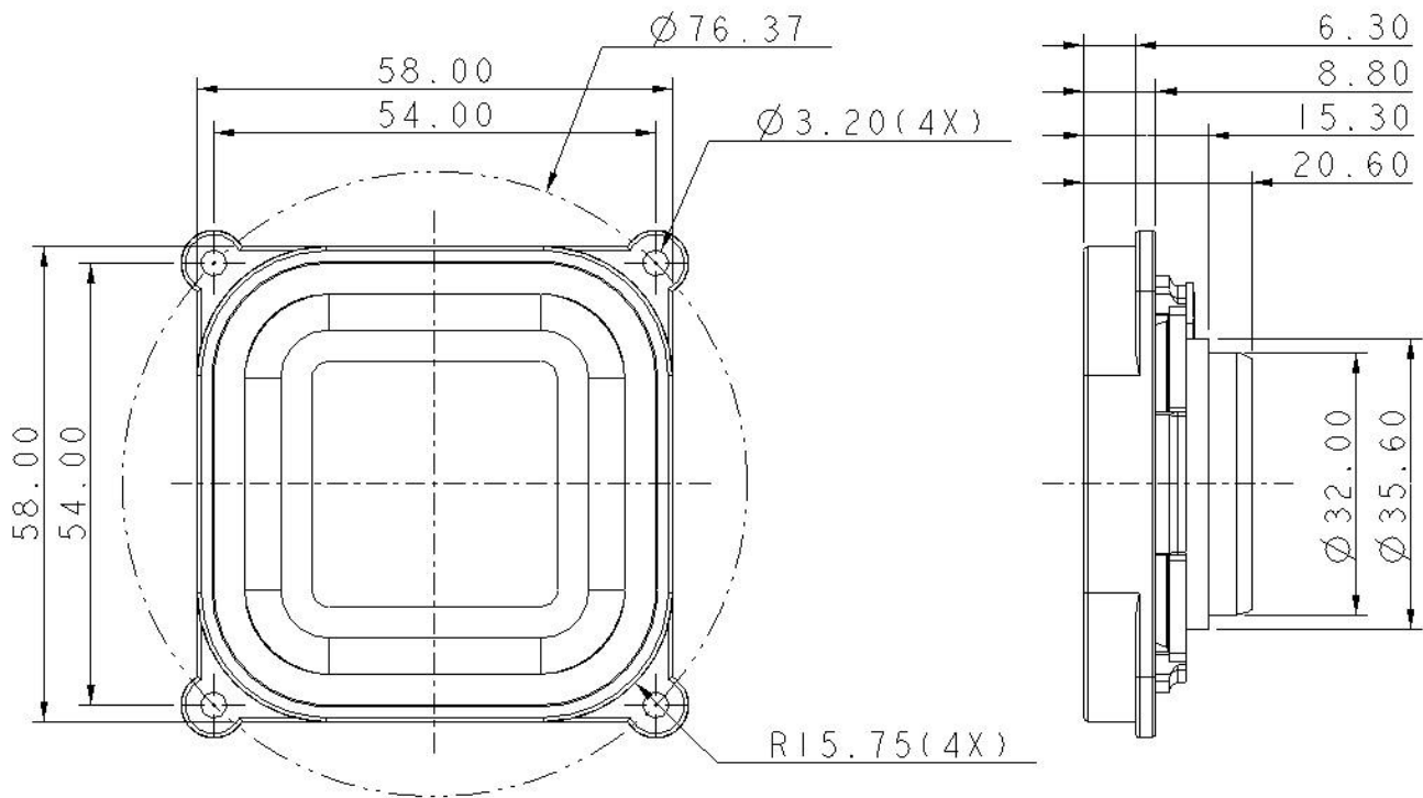
Figure 2. Nominal dimensions
